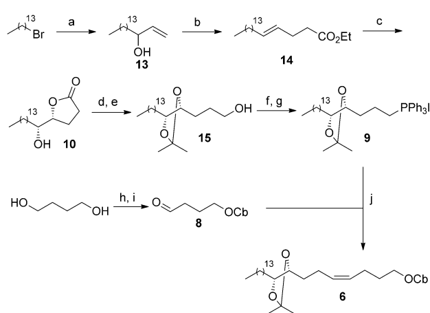
Scheme 4. Synthesis of left-hand fragment, carbamate 6 . a) i) Mg, \text{Et}_2\text{O} , ii) acrolein, 71%; b) \text{CH}_3\text{C}(\text{OEt})_2 , \text{EtCOOH} , PhH, 84%; c) AD-mix- \beta , \text{CH}_3\text{SO}_2\text{NH}_2 , t\text{BuOH}/\text{H}_2\text{O} , 73%; d) \text{LiAlH}_4 , \text{Et}_2\text{O} ; e) \text{C}(\text{CH}_3)_2(\text{OMe})_2 , TsOH, PhH, 75% (over 2 steps); f) \text{PPh}_3 , imidazole, \text{I}_2 ; g) \text{PPh}_3 , MeCN, reflux, 18 h, 84% (over 2 steps); h) NaH, CbCl, THF; i) TCCA, TEMPO, \text{CH}_2\text{Cl}_2 , 82% (over 2 steps); j) 9 , THF, NaHMDS, -78^\circ\text{C} , then 8 , -78^\circ\text{C} to RT, 18 h, 79%. HMDS = 1,1,1,3,3,3-hexamethylidisilazane, TCCA = trichloroisocyanuric acid, TEMPO = 2,2,6,6-tetramethylpiperidine- N -oxyl, Ts = p -toluenesulfonyl.
