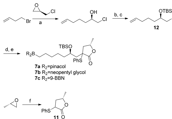
Scheme 5. Syntheses of boronic esters 7 and lactone 11 . a) i) Mg, \text{Et}_2\text{O} , ii) ( R )-epichlorohydrin, CuI, 87%; b) NaI, acetone 89%; c) TBSCl, imidazole, \text{CH}_2\text{Cl}_2 , RT, 40 h, 94%; d) 11 , LDA, 0^\circ\text{C} , 30 min, then 12 , RT, 60 h, 73%; e) \text{R}_2 = pinacol: [\{\text{Ir}(\text{cod})\text{Cl}\}_2] , dppe, (pin)BH \text{CH}_2\text{Cl}_2 , 79%; \text{R}_2 = neopentyl glycol: [\{\text{Ir}(\text{cod})\text{Cl}\}_2] , dppb, \text{CH}_2\text{Cl}_2 (cat)BH; neopentyl glycol, 59%; \text{R}_2 = 9-BBN: 9-BBN, THF, RT, 2 h, (after oxidation at RT for 2 h with \text{NaOAc}/\text{H}_2\text{O}_2 ) 98%; f) i) LDA, \text{PhSCH}_2\text{COOH} , ii) TsOH, PhH, 84% (over 2 steps). 9-BBN = 9-borabicyclo[3.3.1]nonane, cod = cycloocta-1,5-diene, dppb = 1,4-bis(diphenylphosphanyl)butane, dppe = 1,4-bis(diphenylphosphanyl)ethane, LDA = lithium diisopropylamide, pin = pinacol.
