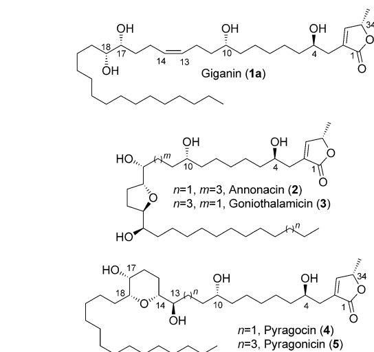
Scheme 1. Annonaceous acetogenins.
